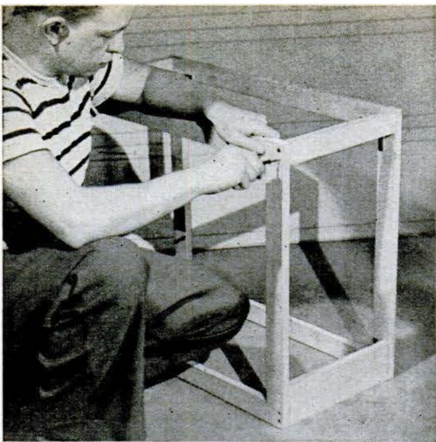
FRAME is made of 1" by 2" pine strips. Here front is being joined to back with crosspieces. Lower crosspieces are double strips.
